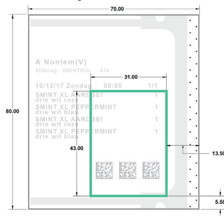
Pouch Layout with Visible Area
